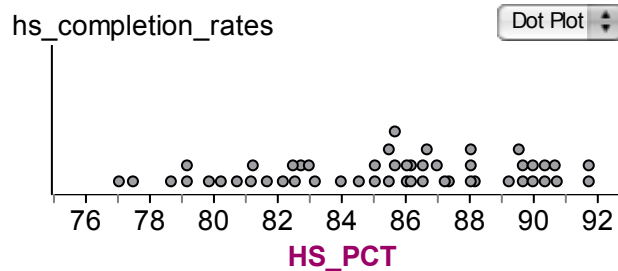
Display D2.9: Dotplot of high school completion rates.
