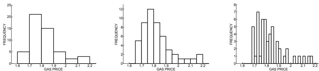
Display D2.26: Histograms of average gasoline prices using bins of width 0.10, 0.05, and 0.02.
